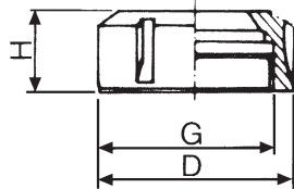
FIG.4 ER25,32,40,50UM
