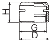
FIG.1 ER11,16,20MS
