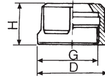
FIG.3 ER11,16,20UM
