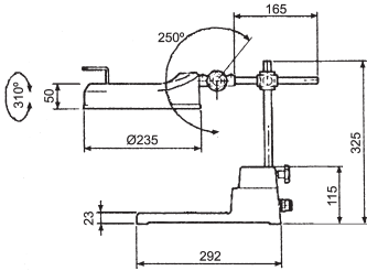
VHL-30TEB BENCH TYPE
