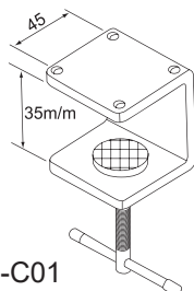
MOUNTING CLAMP
